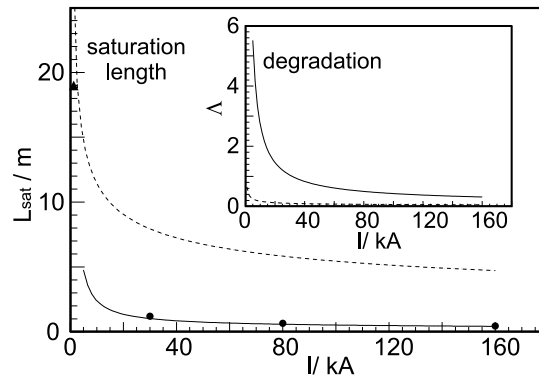
FIGURE 2 Saturation lengths (3) and (inset) degradation factor \Lambda as a function of electron beam current I : DESY's FLASH (dashed curve, triangle) and the table-top VUV scenario (solid line). The circles denote specific GENESIS runs
