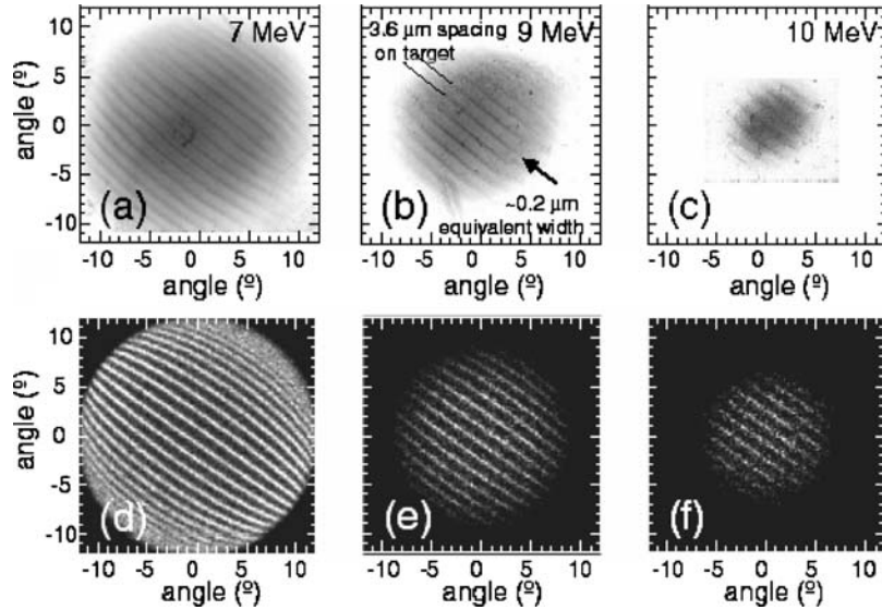
Figure 3. (a–c) Angular distributions on RCF of protons accelerated from an 18- \mu\text{m} thick Al flat target irradiated at 10^{19} W/cm ^2 . (d–f) Simulated RCF images [same parameters and proton energies as in (a–c)] using a 3D PIC effective code.
