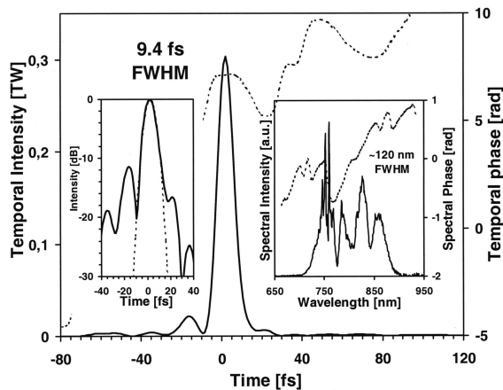
Fig. 4. Pulse shape and spectrum at the output of the three-stage amplifier system (solid curves) with the corresponding phases (dashed curves) measured by SPIDER. Left inset, pulse shape on a logarithmic scale with a Gaussian fit of the same duration (dotted curve).
