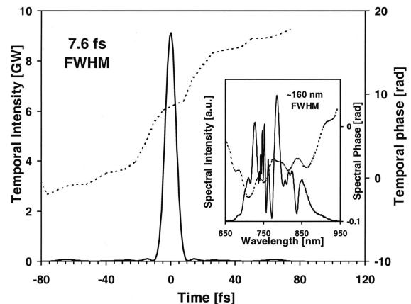
Fig. 3. Pulse shape and spectrum of the compressed fiber output (solid curves) with the corresponding phases (dashed curves) measured by SPIDER.
