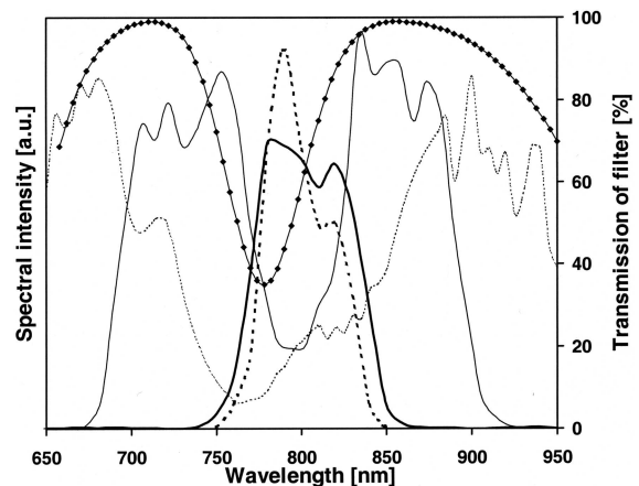
Fig. 2. Output spectrum of the first stage with (solid thick curve) and without (dashed thick curve) spectral filtering, and the transmission of the different spectral filters in the first stage (solid thin curve), in the second stage (dashed thin curve), and the AOPDF (solid curve with diamonds).
