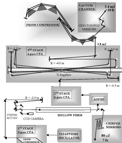
Fig. 1. Experimental setup of the three-stage amplifier system. GDD, group-delay dispersion; TOD, third-order dispersion; FOD, fourth-order dispersion; CPA, chirped-pulse amplification.
