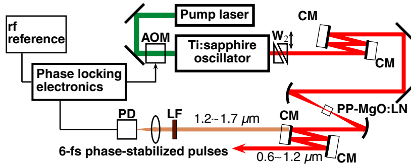
Figure 3. Experimental realization of the monolithic CE-phase stabilization scheme. W_2 , fused silica-wedged plate that may be used for control of the CE-phase and fine adjustment of the chirp. CM, chirped mirror; LF, long-pass filter (cutoff 1400 nm); PD, InGaAs photodiode (NewFocus, 1811-FC), phase-locking electronics (MenloSystems); rf reference, signal generator (Marconi, 2022D: operated at 12.5 MHz); and AOM, acousto-optic modulator.
