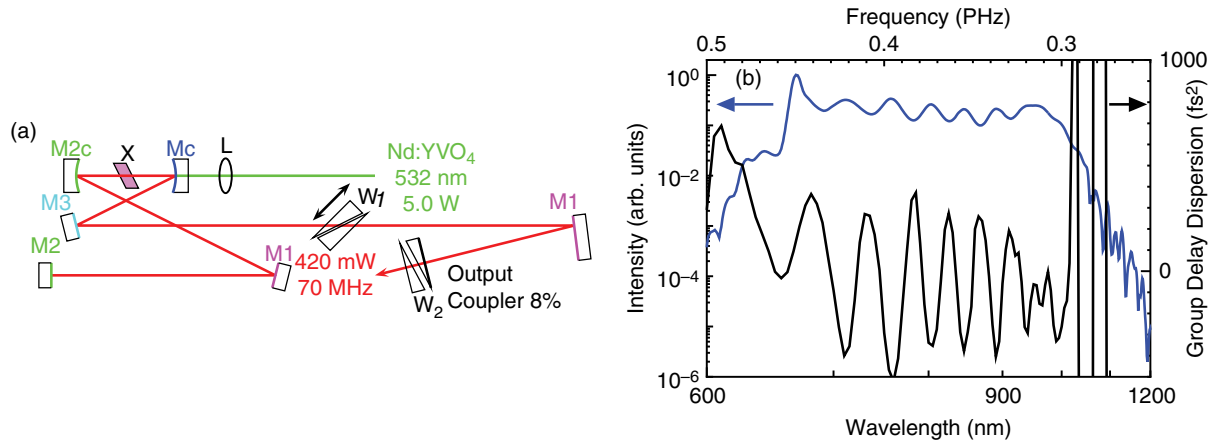
Figure 2. (a) The schematic representation of the broadband Ti:sapphire oscillator. X, Ti:sapphire crystal ( t = 2.6 mm); Mc/M2c, 50 mm ROC folding mirror; M1–M3, chirped mirrors; and L, incoupling lens. The wedged plates inside the laser cavity ( W_1 ) allow the controlling of CEO frequency ( f_{\text{CEO}} ), while extra-cavity wedges ( W_2 ) shift the CE-phase. (b) Spectrum generated by the oscillator (blue curve), measured with a scanning monochromator (Ando, AQ-6315A) and net intracavity group-delay dispersion (GDD, black curve).
