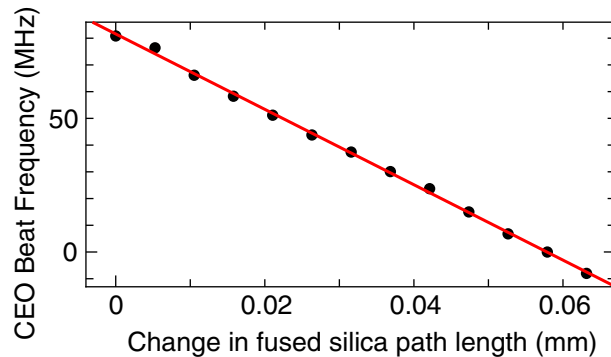
Figure 5. Measured CEO beat signal versus change in round-trip path length through the intracavity-fused silica wedges.
