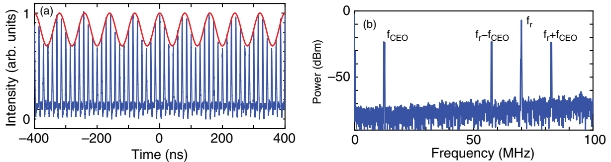
Figure 4. (a) A pulse train from the nonlinear crystal filtered in the wavelength range of longer than 1400 nm is modulated at f_{CEO} (red curve) and monitored with a digital oscilloscope (Tektronix, TDS7104). (b) rf spectrum of the same signal measured with a spectrum analyser (Agilent E4401B). Resolution bandwidth is 100 kHz.
