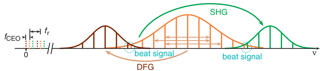
Figure 1. Principle of f_{\text{CEO}} detection: two additional frequency combs, f_k = kf_r and f_m = mf_r + 2f_{\text{CEO}} , are created in a nonlinear crystal by DFG and SHG, respectively. The frequency comb of the seed laser f_n = nf_r + f_{\text{CEO}} , which is spectrally broadened by SPM, is located between the DFG and SHG combs. With k, n and m being integers, the combs partially overlap to produce heterodyne beat notes at f_{\text{CEO}} .
