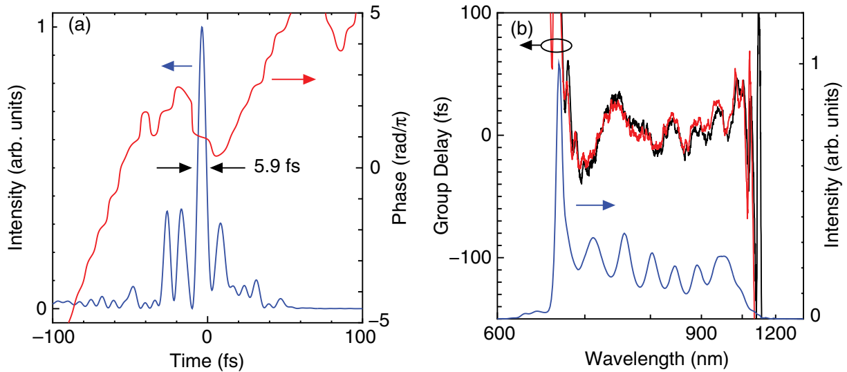
Figure 8. (a) Temporal profile of the output pulses of the phase-stabilized system (passing through the 2 mm length PP-MgO:LN and compressed with chirped mirrors), as retrieved from a SPIDER measurement. The full-width at half-maximum of the intensity profile is 5.9 fs. (b) Group delay (black curve) and spectrum (blue curve, linear scale) of the pulses. The group delay when the beam is not focused on the crystal is also shown as a red curve.
