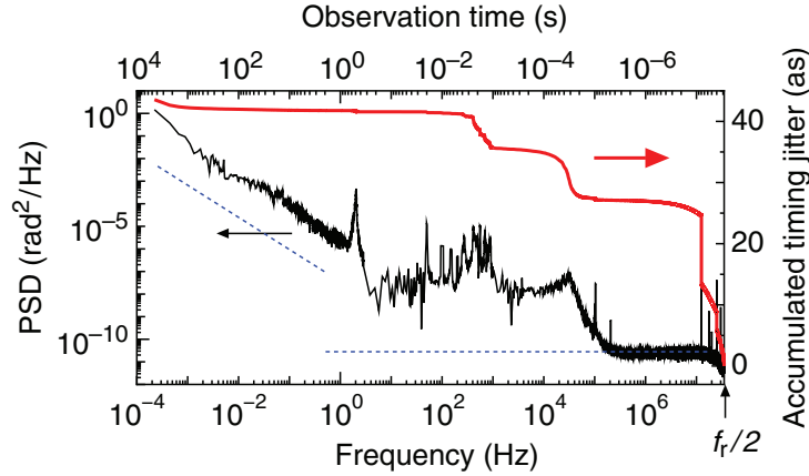
Figure 7. Out-of-loop two-sided phase-noise power spectral density (PSD), S_{\phi}(\nu) and integrated CE timing jitter. The dotted line shows the noise floor of the photo detector and the vector voltmeter for low frequencies. The large peaks in the high frequency region (12.5, 17.5, 20, 25, 30 MHz) are originated from rf pick up.
