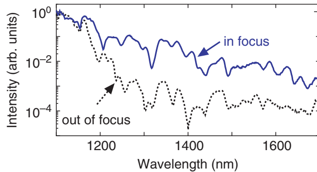
Figure 6. The long-wavelength tail of the laser spectrum exiting from the nonlinear crystal, measured with an optical spectrum analyser (Ando, AQ-6315A). The solid line shows the optimized spectrum, whereas the dotted line depicts it with the crystal shifted out of focus, for reference.
