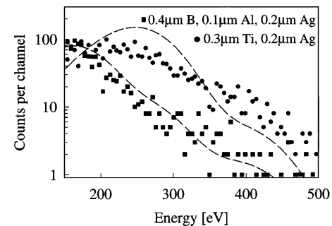
FIG. 5. Energy spectra transmitted through different filter combinations for 7-fs pump pulses. Correction of the near-field XUV radiation spectrum from Fig. 2 for the detector response and respective filter (and window) transmittances result in the dotted lines (without using fit parameters).
