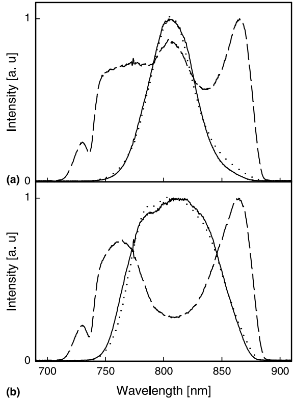
Fig. 6. Amplified and unamplified spectrum (a) without spectrum shaping and (b) with spectrum shaping.
