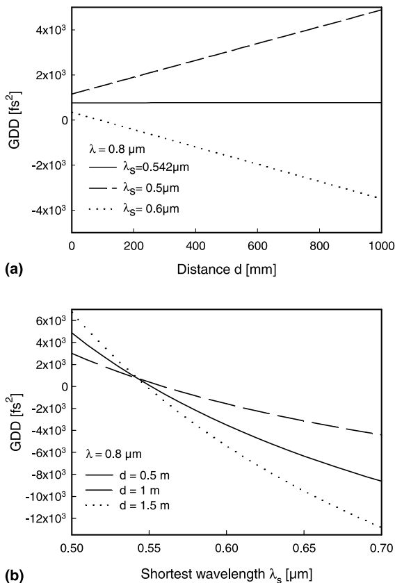
Fig. 2. (a) GDD (at \lambda_0 = 0.8 \mu\text{m} ) as a function of d . (b) GDD (at \lambda_0 = 0.8 \mu\text{m} ) versus the shortest wavelength \lambda_s .
