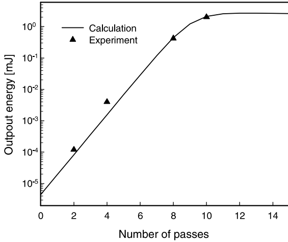
Fig. 5. Output energy as a function of pass number.
