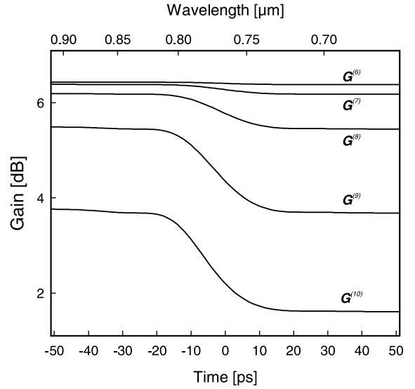
Fig. 4. Instantaneous gain for last five passes.
