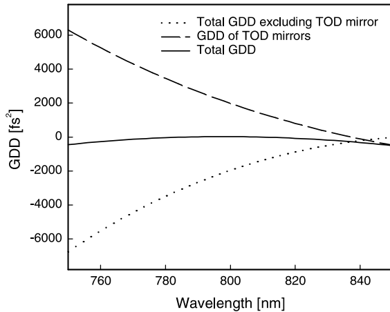
Fig. 10. Group-delay dispersion of the system.
