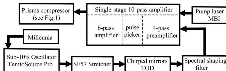
Fig. 7. Schematic of the laser system.
