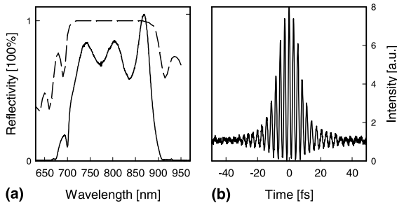
Fig. 8. (a) Seed pulse spectrum (full line). (b) Interferometric autocorrelation of seed pulse.
