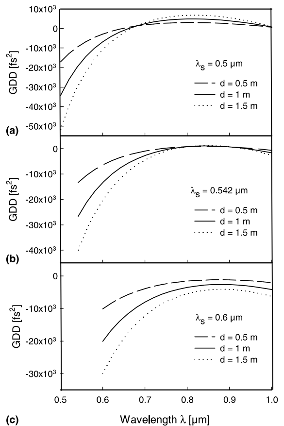
Fig. 3. GDD versus wavelength.
