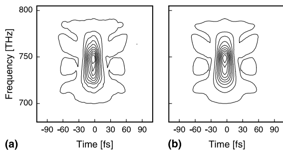
Fig. 11. (a) Measured and (b) retrieved FROG trace of a 17.5 fs pulse. The contour plots depict iso-intensity lines at the levels of 0.01 \times S_p and integer multiples of 0.1 \times S_p , where S_p is the peak of S(\omega, \tau) .
