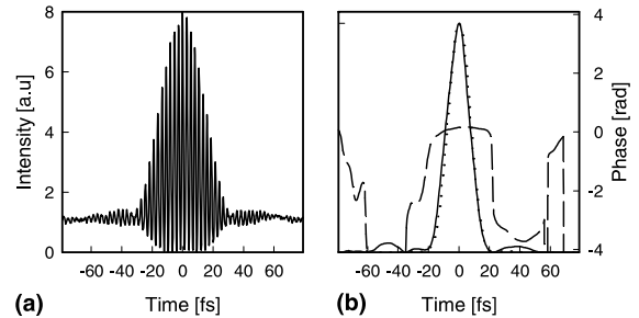
Fig. 12. (a) Interferometric autocorrelation of amplified pulse. (b) Retrieved pulse shape (full line), phase (dashed line) and transform-limited pulse shape (dotted line) from the measured spectrum.
