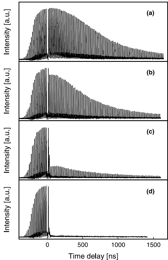
Fig. 9. The evolution of the train of pulses pre-amplified in first four passes through the amplifier: (a) the selected pulse (missing) has not been amplified in additional passes; (b) the selected pulse (missing) has been amplified in additional four passes (eight passes); (c) in additional five passes (nine passes) and (d) in additional six passes (10 passes).
