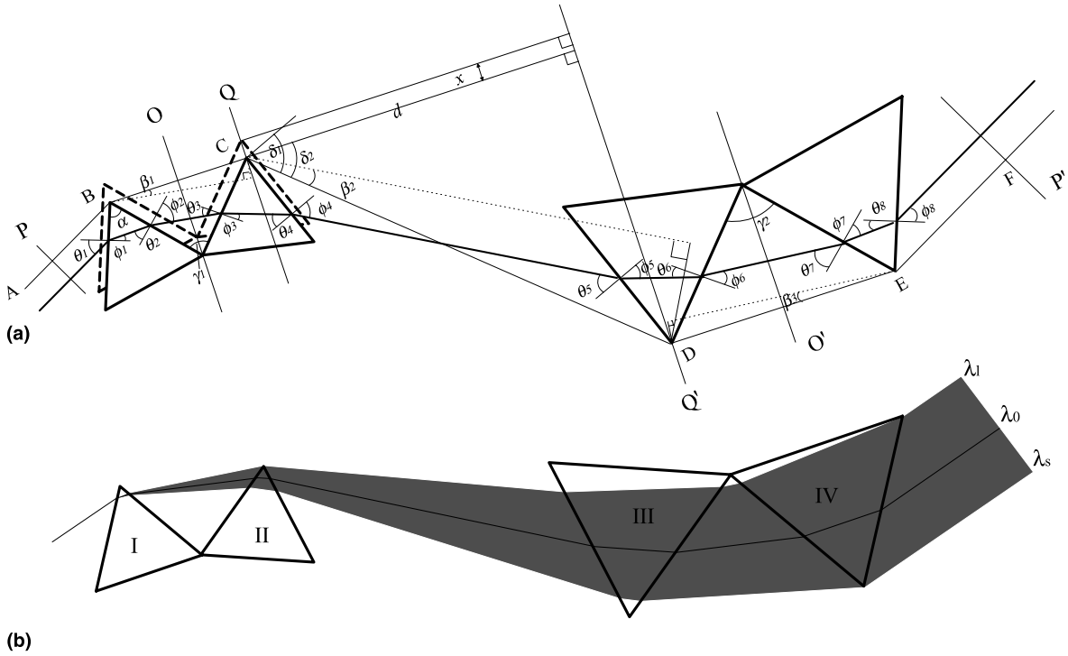
Fig. 1. Diagram of a pair of double prisms.
