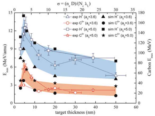
Fig. 1. (Color online) Maximum energy per atomic mass unit for both protons and carbon ions plotted vs. foil thickness for values of the normalized laser vector potential of a_0 = 3.6 and a_0 = 5 . The experimental results are in excellent agreement with numbers deduced from 2D-PIC-simulations.
