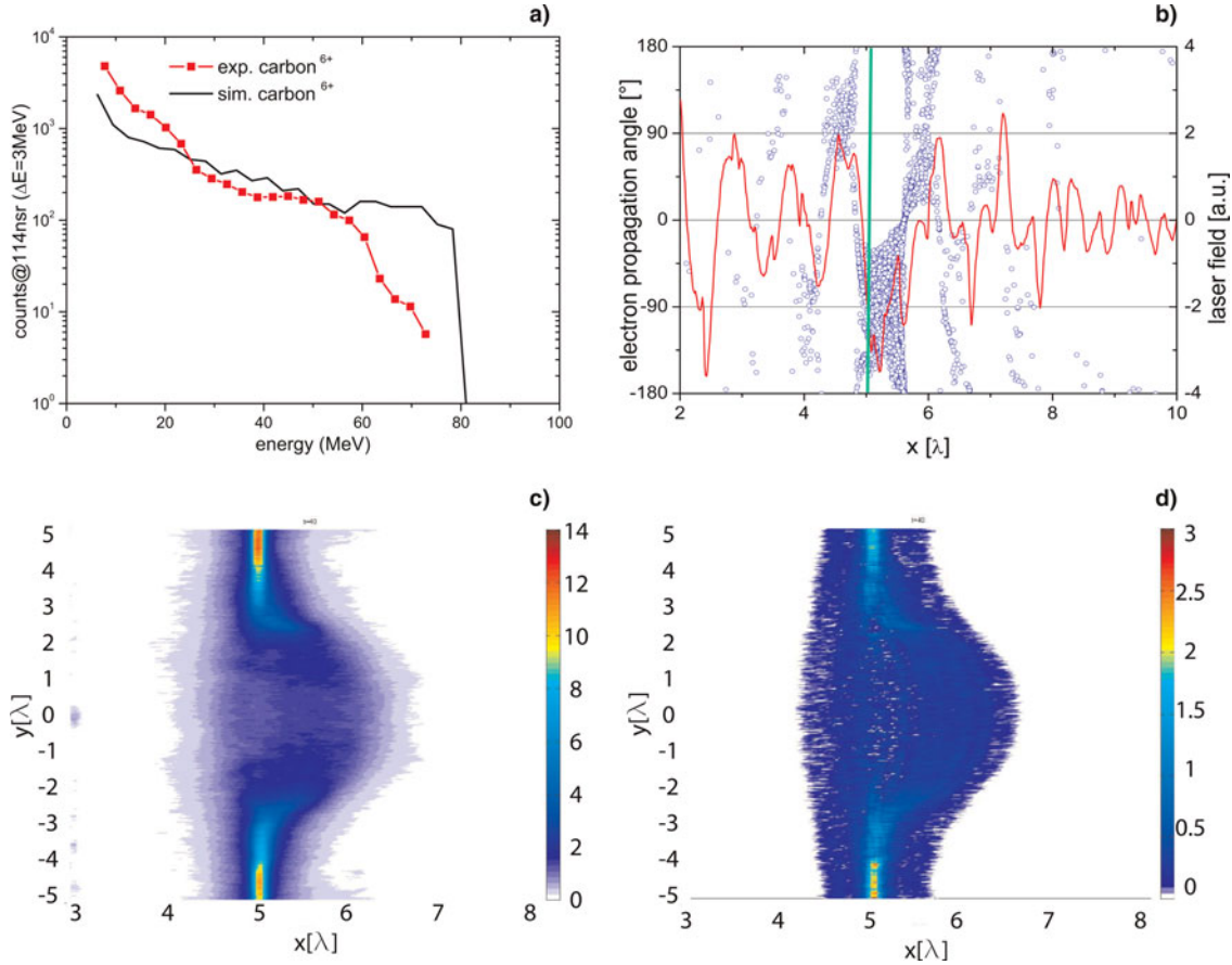
Fig. 4. (Color online) (a) Comparison between experimentally obtained and simulated C^{6+} spectrum as deduced from a 2D-PIC simulation of a 4.5 nm foil target (b) Electron propagation angle (blue circles) and laser transverse electric field E_y (red line), plotted vs. laser propagation direction x , given in units of the laser wavelength \lambda . \tau is given in laser cycles. The green line at x = 5\lambda gives the initial location of the target. For the same simulation, (c) gives the electron and (d) the carbon density distribution vs. x at time t = 40\tau .
