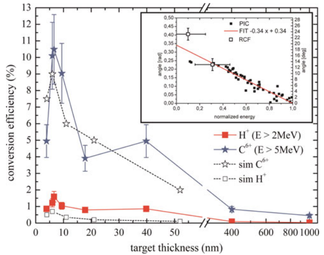
Fig. 2. (Color online) Calculated CE for protons and C^{6+} ions as a function of the target thickness, based on an energy dependent divergence angle of the ion beam, which was extracted from PIC simulations and supported by measured beam profiles (cf. figure inset). The experimental data are in good agreement with the values of the CE obtained from PIC simulations.
