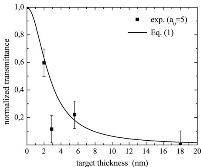
Fig. 3. Measured laser pulse ( a_0 = 5 ) transmittance of the DLC targets as a function of the target thickness compared to the analytical model of Vshivkov et al. (1998), Eq. (1).
