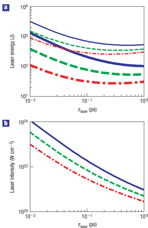
Figure 6 Projections of required laser energy and intensity to achieve a certain proton maximum energy using the adjusted fluid model. a , Required laser energy in the focal spot to achieve 200 MeV as maximum proton energy for various laser pulse durations and target thicknesses (blue solid line, 25 \mu\text{m} ; dashed green line, 10 \mu\text{m} ; dash-dotted red line, 2 \mu\text{m} ). The thinner lines are for a 10 \mu\text{m} FWHM focal spot, and the thicker lines are for a 3 \mu\text{m} FWHM focal spot. b , The required laser intensity to achieve the same goal with the same parameters. The influence of the focal spot diameter is less apparent on the required intensity.
