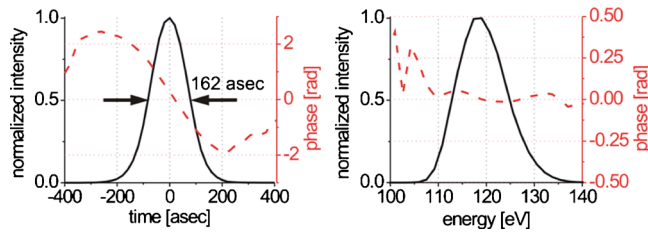
FIG. 7. (Color online) (a) Retrieved temporal intensity (solid line) and phase (dashed line) of the XUV pulse. (b) Retrieved spectrum (solid line) and spectral phase (dashed line) of the XUV pulse.
