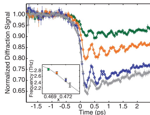
Fig. 1. Bismuth (111) x-ray diffraction efficiency as a function of time delay between the optical excitation pulse and x-ray probe for excitation fluences of 0.7 (green), 1.2 (red), 1.7 (blue), and 2.3 mJ/cm 2 (gray). The zero-delay point was set at the half maximum of the initial transient drop. The inset displays the optical phonon frequency as a function of the normalized atomic equilibrium position along the body diagonal of the unit cell x as measured by x-ray diffraction. The dotted curve represents the theoretical prediction obtained from DFT calculations of the excited-state potential-energy surface (10).
