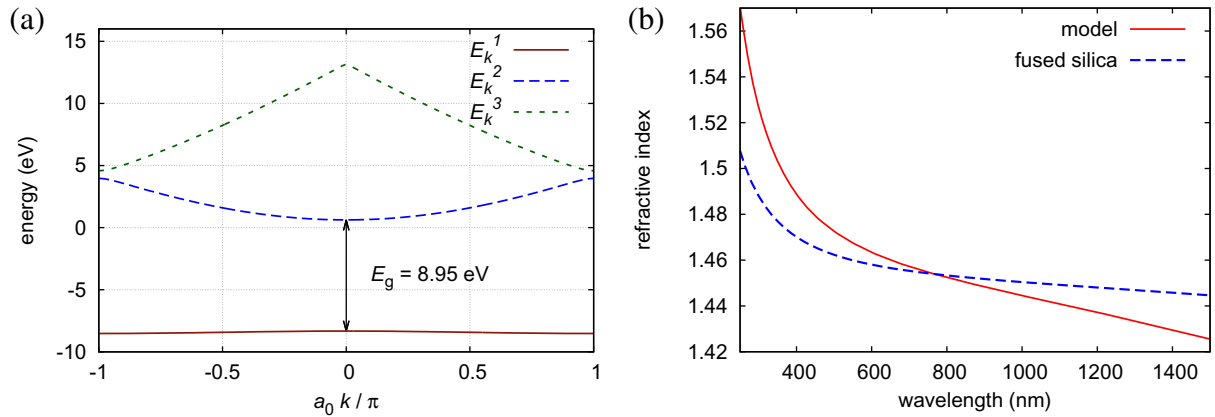
Figure 1. (a) The uppermost valence band and the two lowest conduction bands of the model potential (21). (b) A comparison of the refractive index evaluated according to (24) with the refractive index of fused silica [27].
