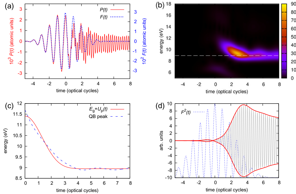
Figure 2. (a) The polarization P(t) induced by a laser pulse with \omega_L = \omega_g/4 ( \lambda_L = 557 nm), a peak intensity of 3 \times 10^{13} \text{ W cm}^{-2} , and \varphi_{\text{CEP}} = 0 . The electric field F(t) is shown by the dotted blue line; the FWHM of the pulse corresponds to the time range from -1.5 to 1.5 optical cycles. (b) S(t, \omega) , which is the result of applying the wavelet transform to P(t) . The dashed white line marks the energy E_g = \hbar\omega_g . (c) The solid red line is the sum of the bandgap energy E_g and the ponderomotive energy U_p(t) . For each time t , the dashed blue line depicts the above-bandgap frequency where S(t, \omega) has a maximum. (d) The quantum-beat part of the polarization response \mathcal{F}^{-1}[\tilde{w}(\omega)\tilde{P}(\omega)] (grey) and its envelope (red). The spectral window used for the analysis is given by (28).
